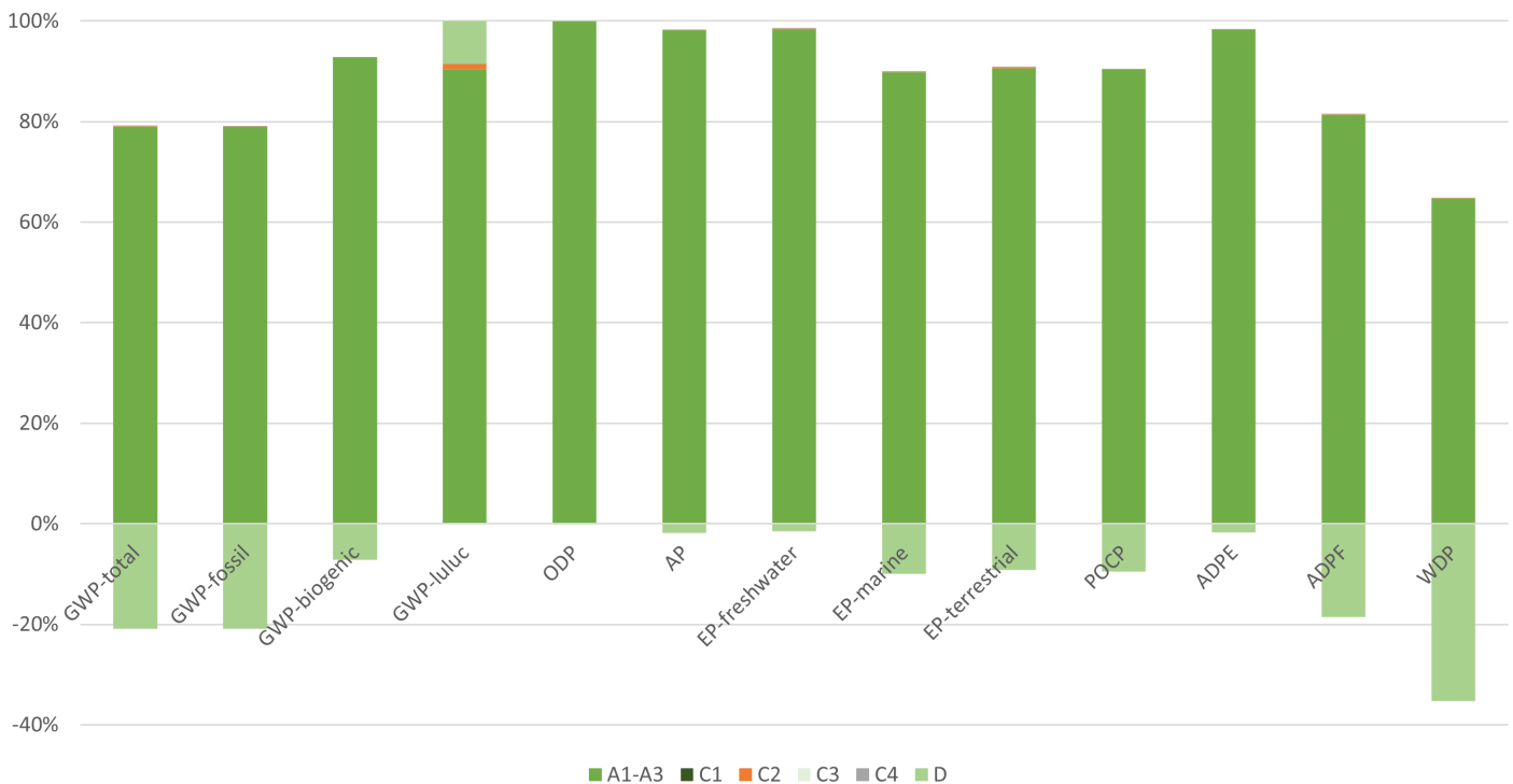
Hot-spot analysis of voestalpine roll-bonded clad plates (UNS N08825 / 2.4858)
