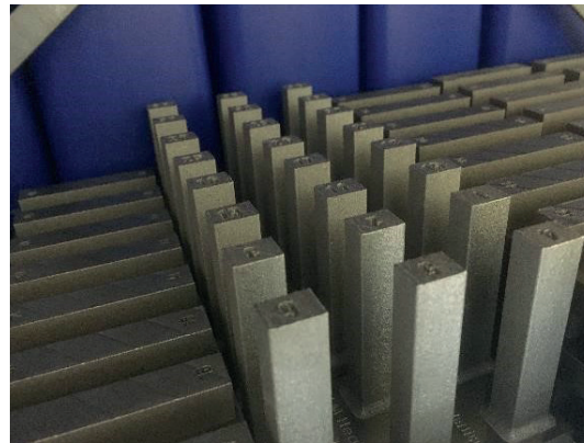
Uddeholm Dievar for additive manufacturing vs 1.2709 and AM H13, printed vertical direction and heat treated to hardness range of 46-48 HRC. The fine grain structure of Uddeholm Dievar for additive manufacturing results in superior high toughness values.
